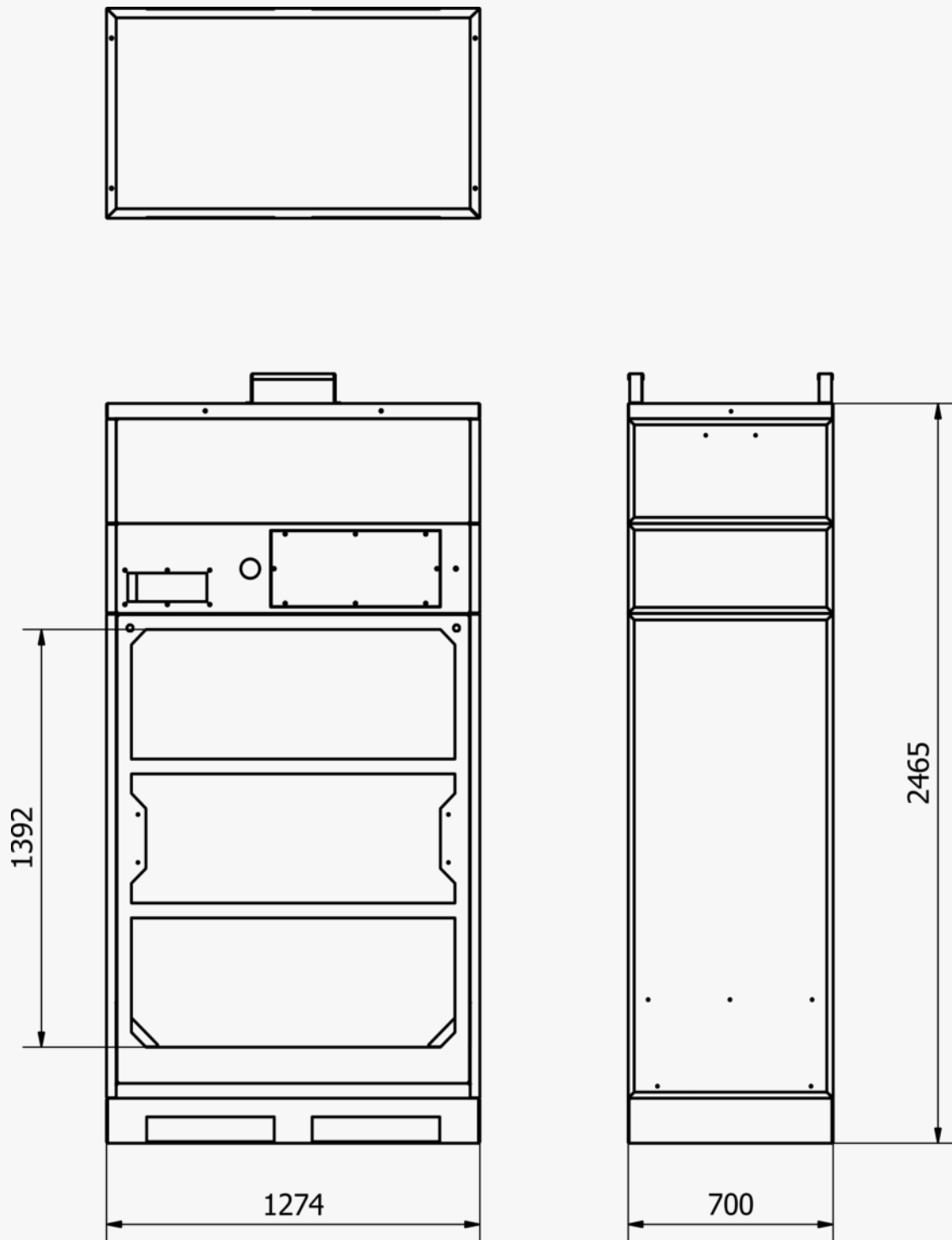
VP121224L Shown - Note ML type also includes HEPA outlet unit
